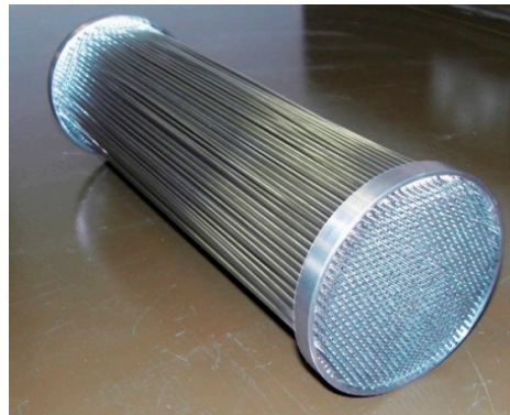
Figure 8. Heat exchanger core of ammonia/carbon heat pump generator [35].
