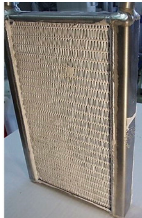
Figure 4. Flat tube–fin coated adsorber [28].
